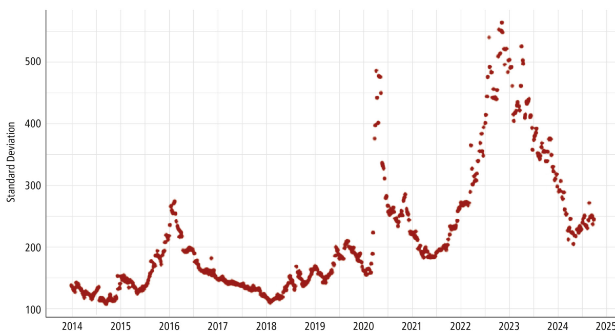
Figure 2: Eurobond spreads: development of the standard deviation
